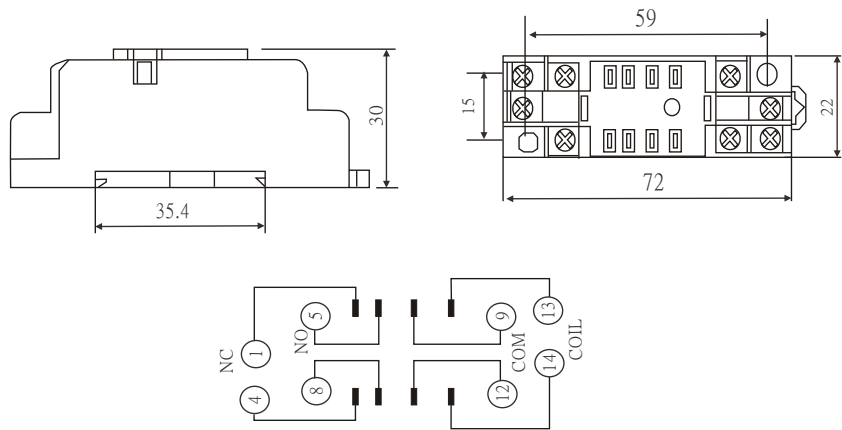
PYF-14A-A Fit to LB4H SERIES
