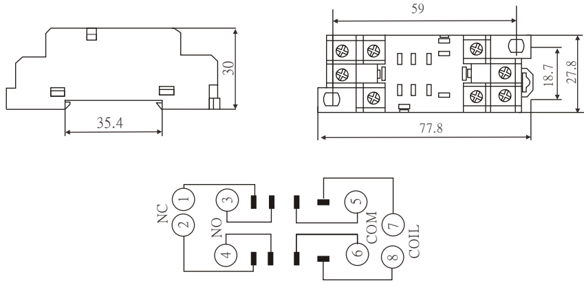
PYF-08A-A Fit to LB2H SERIES
