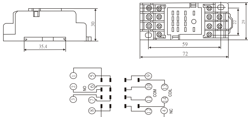
PYF-14A-A Fit to LB4H SERIES
